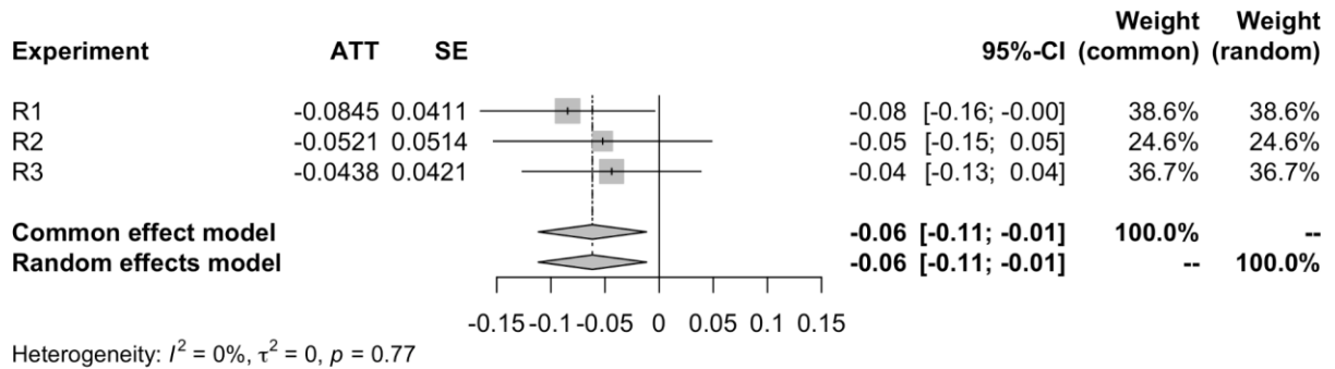
Figure S20. Treatment effect (ATT) on reduction in misinformation sharing and meta-analytic effect. Experiments R1 and R3 used a graded approach to scoring domain quality. The outcome and pre-treatment variables are winsorized at the 99th percentile.
