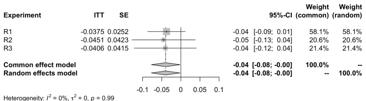
Figure S22. Treatment effect (ITT) on reduction in misinformation sharing and meta-analytic effect. Experiments R1 and R3 used a graded approach to scoring domain quality. The outcome and pre-treatment variables are not winsorized.
