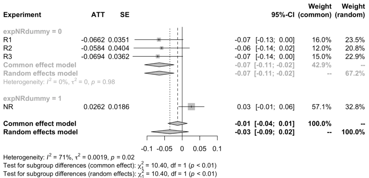
Figure S11. Treatment effect (ATT) on reduction in misinformation sharing and meta-analytic effect. Experiment NR targeted relatively inactive users who had not recently shared links to low quality new sites, but who had done so further in the past.
