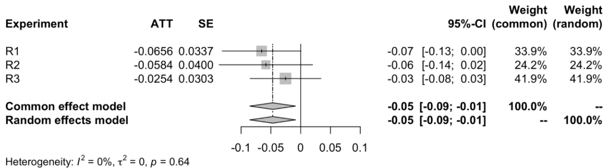
Figure S14. Treatment effect (ATT) on reduction in misinformation sharing and meta-analytic effect. Experiments R1 and R3 used a graded approach to scoring domain quality. Experiment R2 counted the number of relevant low quality hashtags shared.
