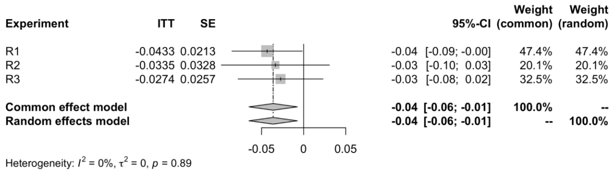
Figure S19. Treatment effect (ITT) on reduction in misinformation sharing and meta-analytic effect. Experiments R1 and R3 used a graded approach to scoring domain quality. The outcome and pre-treatment variables are winsorized at the 99th percentile.
