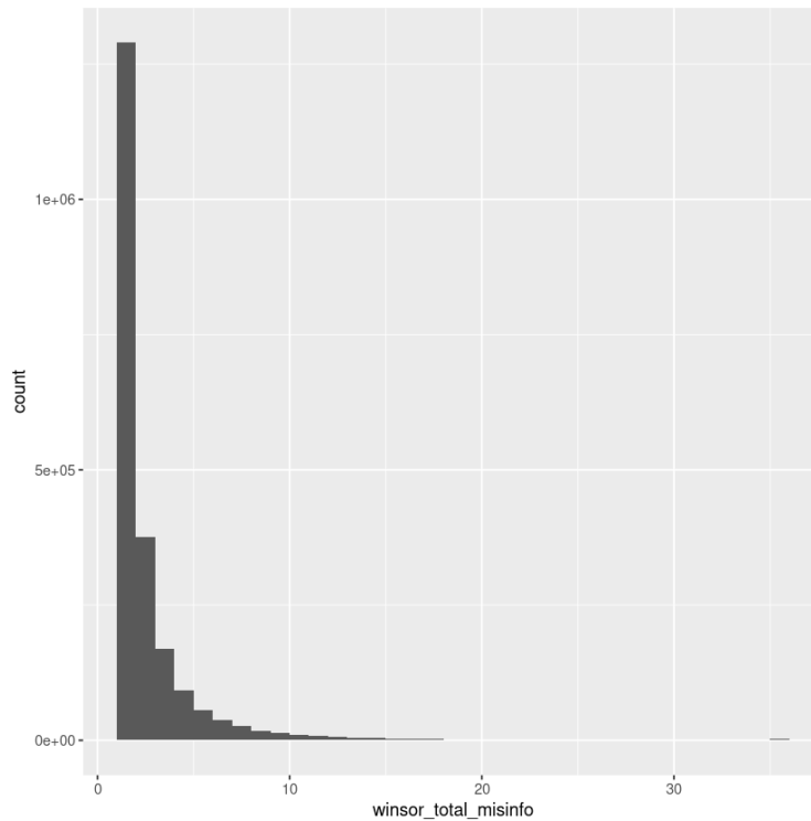
Figure S2. Distribution of the number of pieces of misinformation shared in the pre-experiment week. The x-axis is clipped at the 99.9th percentile (i.e., users that shared more than 36 pieces of misinformation).
