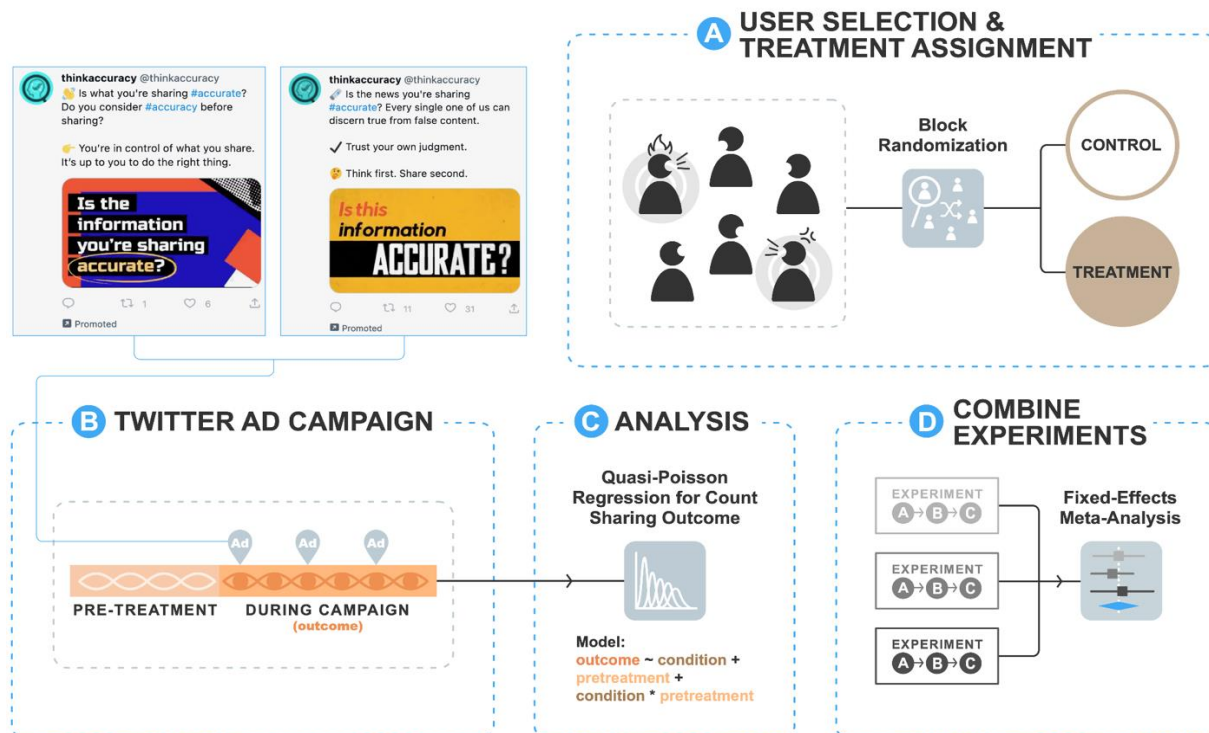
Fig. 3. Twitter study experimental design. The Twitter study targeted highly active users who recently shared low-quality content. The amount of low-quality content shared by users was measured before and during the ad campaign. Results from three separate experiments were combined using fixed-effects meta-analysis.
