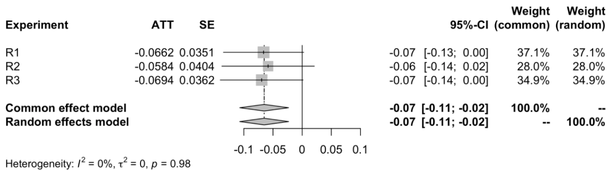
Figure S8. Treatment effect on the treated (ATT) on reduction in misinformation sharing and meta-analytic effect.
