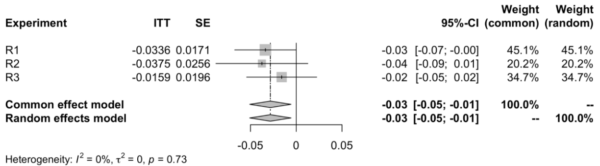
Figure S13. Treatment effect (ITT) on reduction in misinformation sharing and meta-analytic effect. Experiments R1 and R3 used a graded approach to scoring domain quality. Experiment R2 counted the number of relevant low quality hashtags shared.
